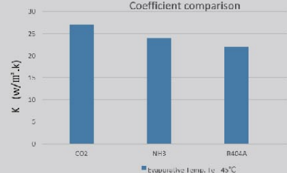
传热系数对比 Coefficient comparison
